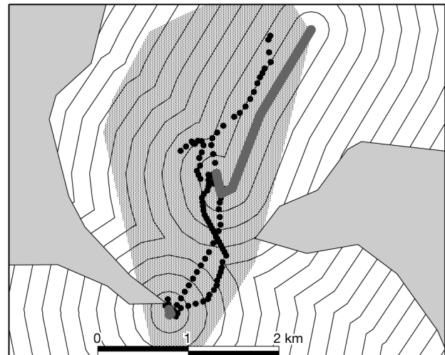
Fig. 7. Tursiops truncatus . An example dolphin track with points interpolated at 44 s intervals (●). The location of the fronts during this period are shown as grey lines, the surrounding lines indicate distances at 200 m intervals and the area considered as available habitat during the dolphin track is shaded
