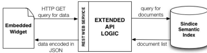
Fig. 1. Message flow in the Sindice Widgets solution.
