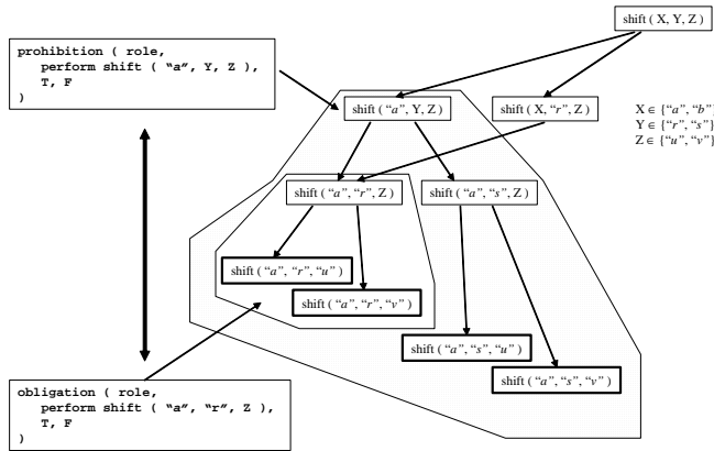
Figure 3. Containment Relationship between Obligation and Prohibition.
