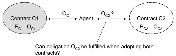
Figure 2. Agent Signs an Additional Contract.
