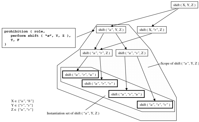
Figure 1. Instantiation Graph and Scope of Influence of Norms.
