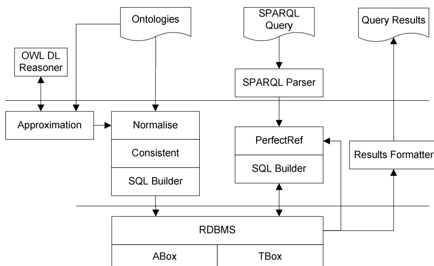
Figure 2: ONTOSEARCH2 system architecture
