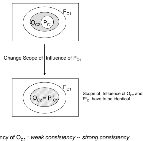
Fig. 5. Introducing a Permission to achieve a state of Strong Consistency.
