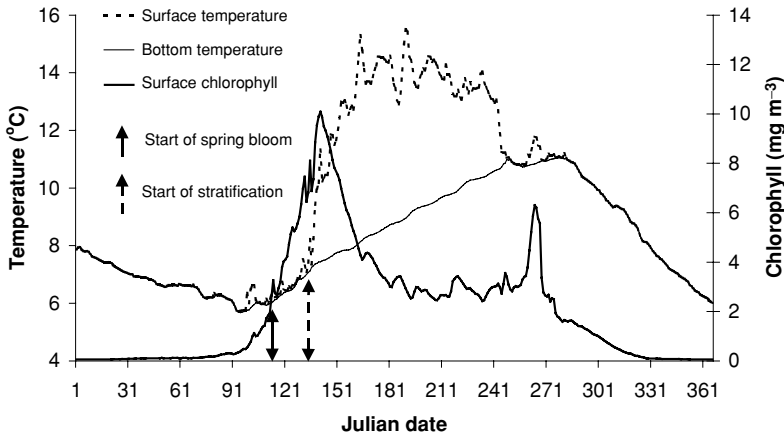
Fig. 4.1 An example of daily output of surface chlorophyll, surface temperature and bottom temperature from the one-dimensional physical-biological model for 1992. The solid arrow marks the timing of the start of the spring bloom, defined as the date when chlorophyll levels exceed 2 \text{ mg m}^{-3} and stay above that value for five consecutive days. The dashed arrow marks the timing of the start of stratification, defined as the date when the difference between top and bottom temperatures exceeds 0.5 \text{ }^{\circ}\text{C} and stays above that value for five consecutive days.
