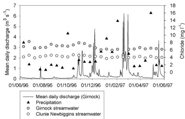
Figure 6 Examples of chloride time series (1996–1997) in the Girnock (example for variable streamwater signature) and Clunie, Newbiggin (example for damped streamwater signature).
