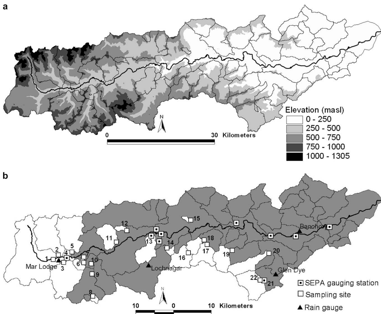
Figure 1 Catchment characteristics of the Dee catchment: (a) topography and (b) catchments investigated and sampling network.
