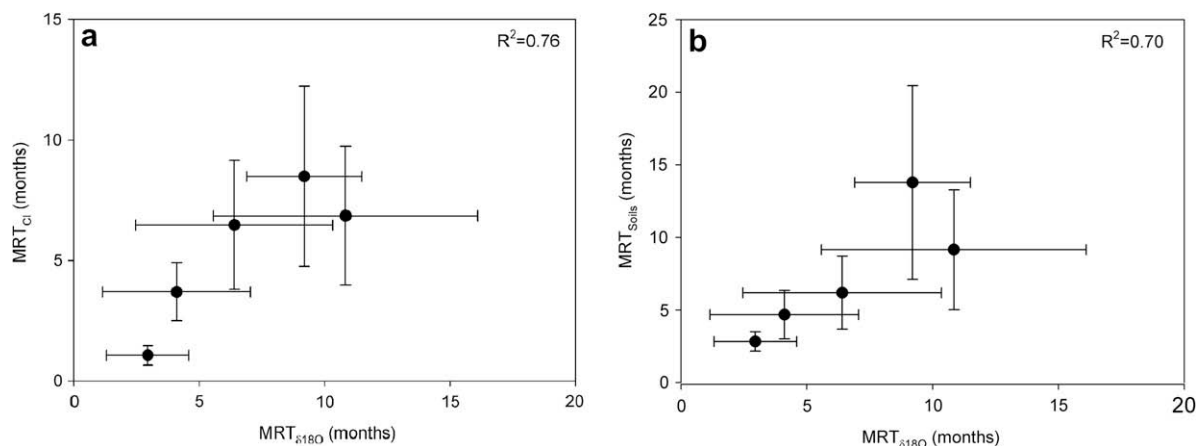
Figure 8 Correlations of (a) MRT_{Cl} predicted from Cl standard deviations and MRT_{\delta^{18}O} and (b) MRT_{soil} and MRT_{\delta^{18}O} . The MRT_{\delta^{18}O} estimates were derived from earlier work in the Feugh (Rodgers et al., 2005b) and Girnock (Tetzlaff et al., 2007b).
