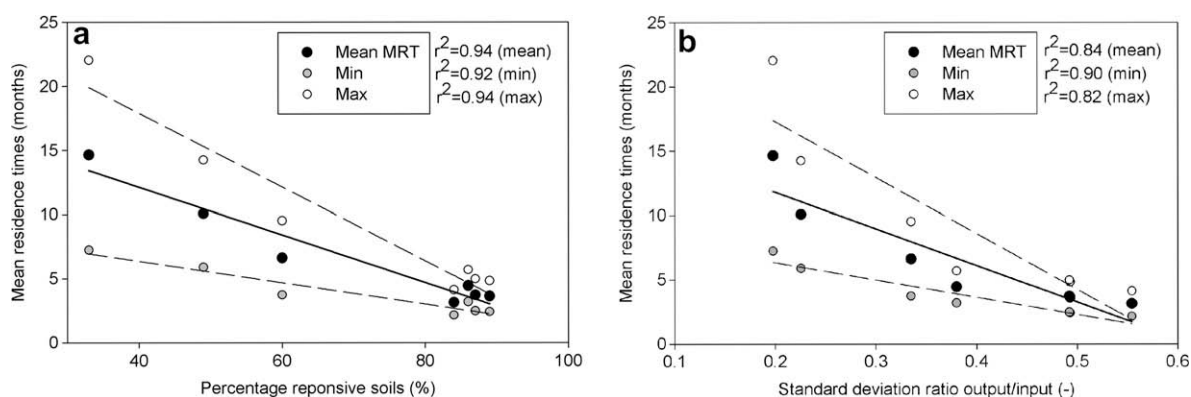
Figure 3 Relationship between (a) \delta^{18}\text{O} based MRT and percentage soil cover in the Feshie and its sub-catchments and (b) \delta^{18}\text{O} based MRT and standard deviation ratios of stream water: precipitation.
