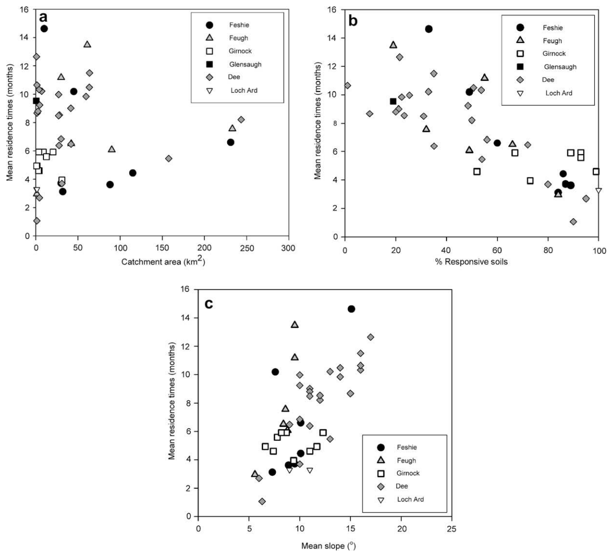
Figure 11 Regionalised relationships between MRT and (a) catchment size, (b) soil cover and (c) mean slope in the Dee sites and others in the Scottish Highlands. MRTs at other sites were estimated from sine wave or convolution integral approaches.
