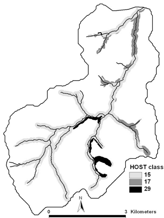
Figure 5 Girnock catchment, HOST classification in riparian zone – defined as 50 m either side of the stream (HOST class 15: Peaty Podzols and Peaty Gleys; HOST class 17: Humus Iron Podzol; HOST class 29: Blanket Peats).
