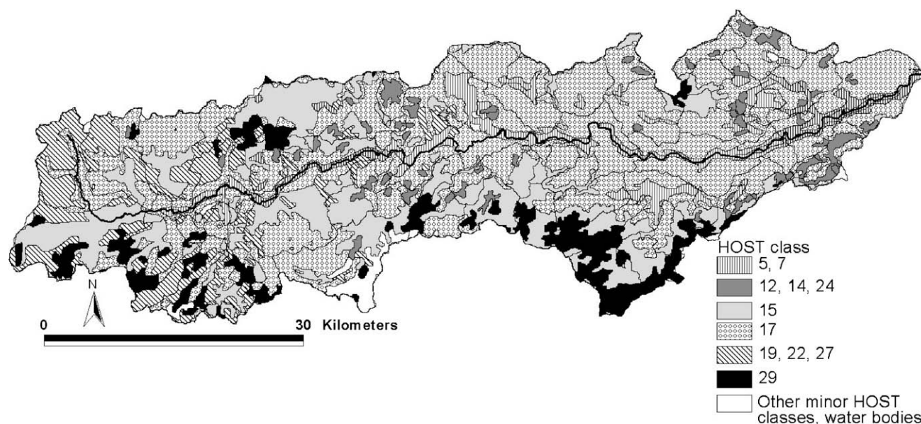
Figure 2 HOST classes of the Dee catchment (HOST classes 5, 7: alluvial soils; HOST classes 12, 14, 24: gleysols; HOST class 15: peaty podzols and peaty gleys; HOST class 17: humus iron podzol; HOST classes 19, 22, 27: rankers; HOST class 29: blanket peats).
