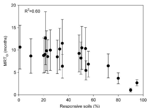
Figure 7 Relationship between MRT_{Cl} and percentage cover of responsive soils.
