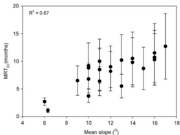
Figure 10 Relationship between MRT_{Cl} and mean catchment slope.
