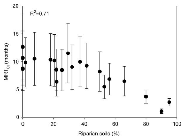
Figure 9 Relationship between MRT_{Cl} and percentage cover of responsive soils in the riparian zone.
