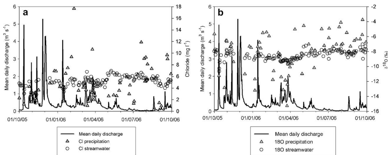
Figure 4 (a) Cl and (b) \delta^{18}\text{O} in weekly precipitation and streamwater samples in the Girnock tributary of the Dee catchment.
