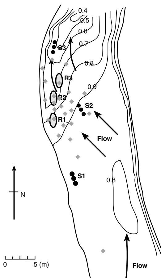
Figure 3. The Gironck Burn field site showing equipment and sampling locations, relative to previous spawning locations (1991–1999 ♦), streambed topography (0.1 m intervals) and direction of water movement: S (●) denotes the site of a piezometer nest; R denotes an artificial redd location
