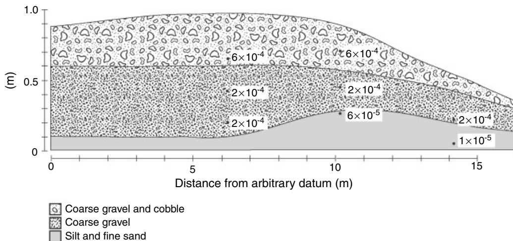
Figure 4. Longitudinal cross-section through spawning riffle showing the spatial variability of hydraulic conductivity ( \text{m s}^{-1} ). Conductivity values presented at location of determination
